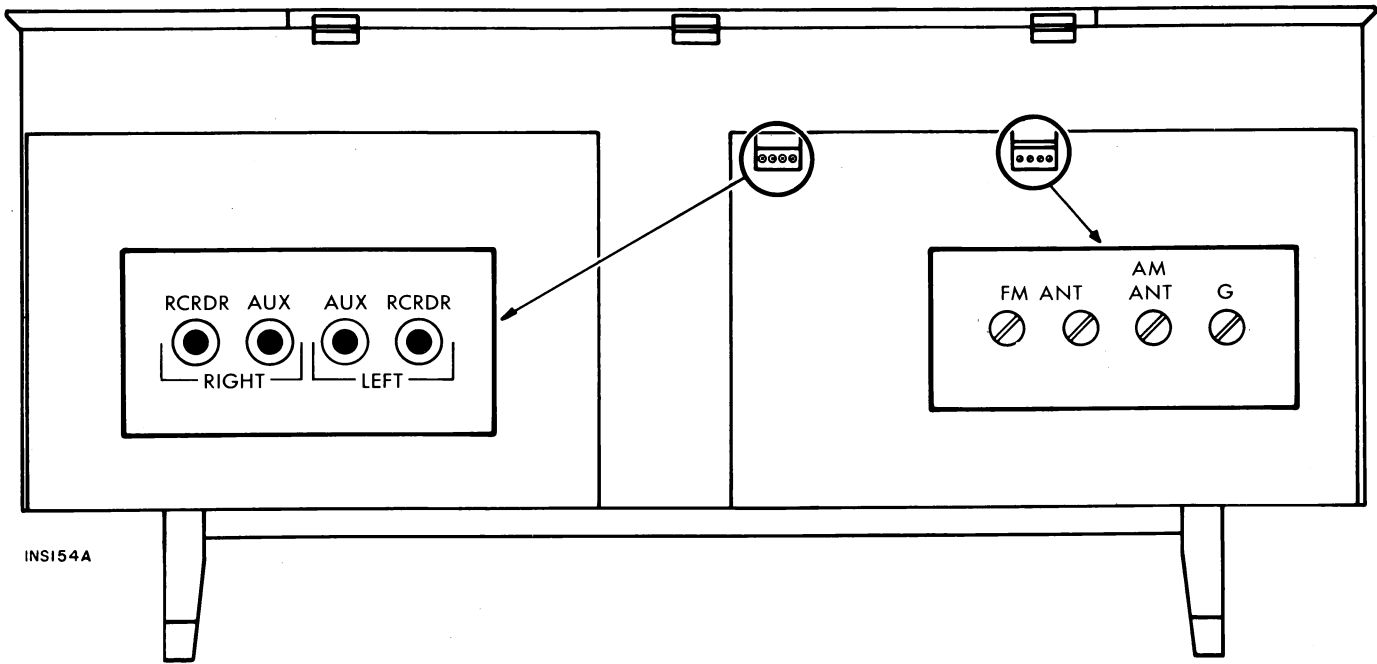
FIGURE 1. Rear View of the Diplomat
